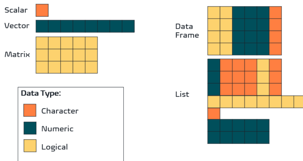
Figure 1. Visual representation of various object types that data may be stored in within R. Note that scalars, vectors, and matrices may contain any type of data so long as only one type is used throughout. For example, this figure displays a matrix of logical data, but matrices are not limited to only logical data. A matrix can contain character, numeric, or logical data; the only restriction is that all data is of the same type.
