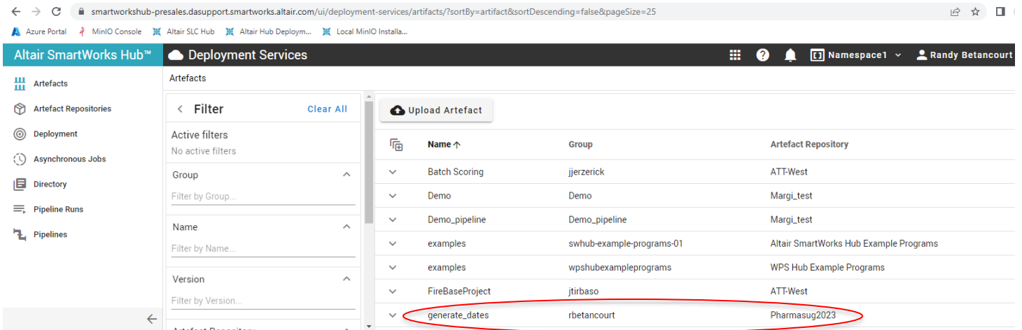
Figure 7. Artifact “generate-dates”
