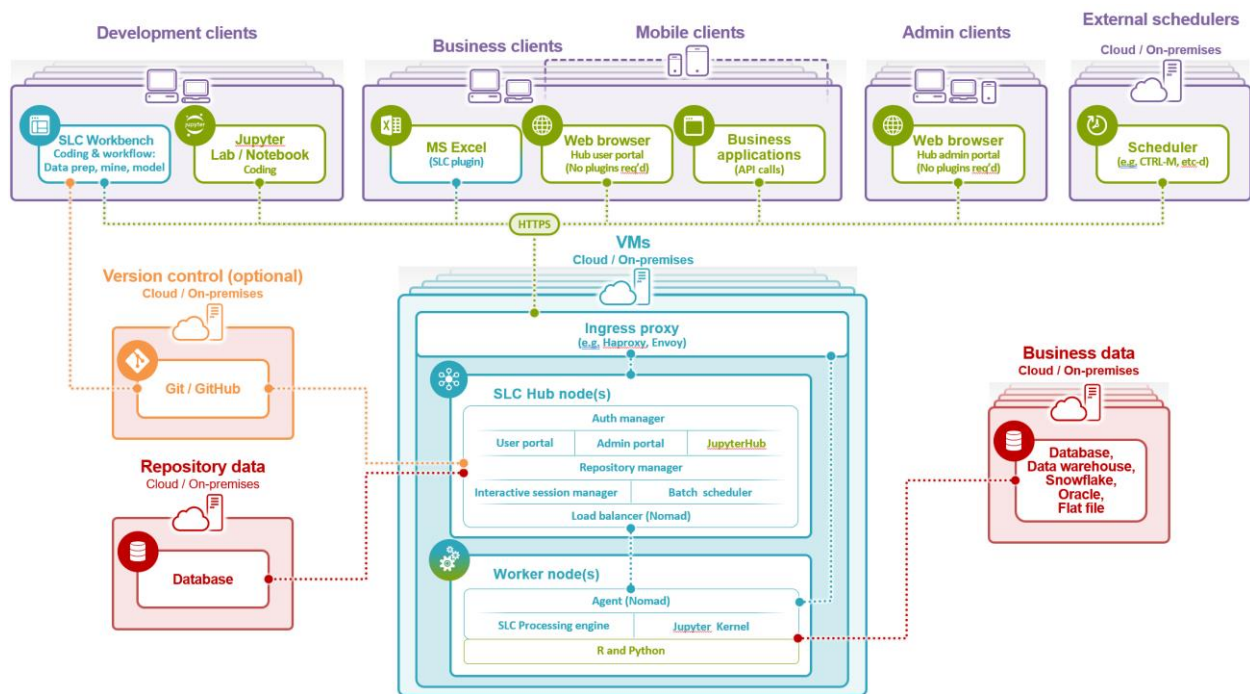
Figure 1. SLC Hub Architecture
