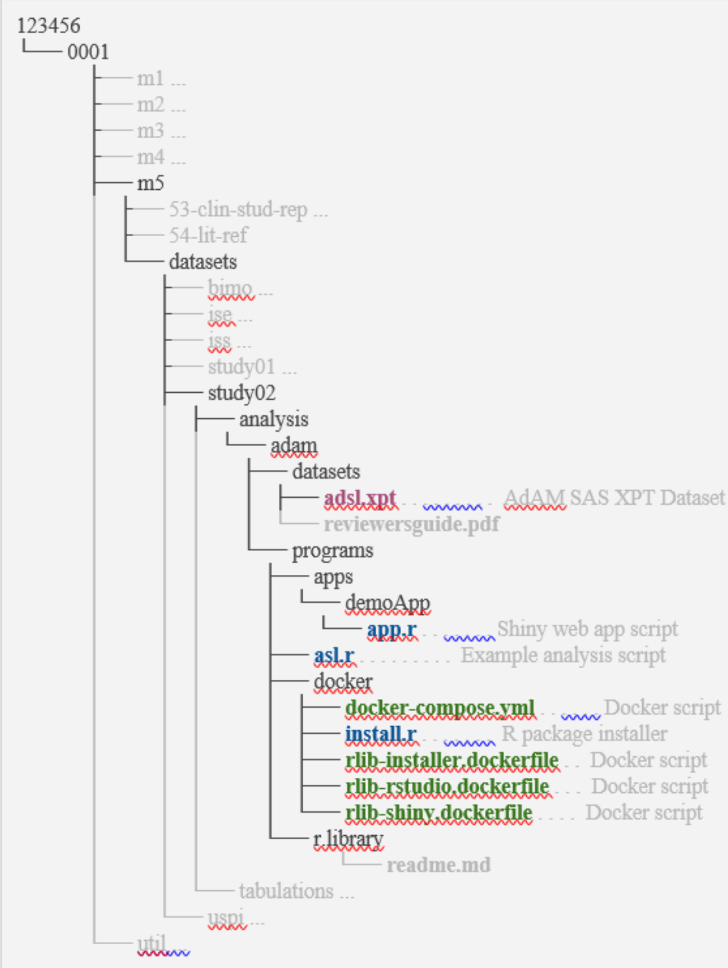
Figure 1: How Docker files fit into eCTD structure
