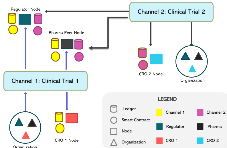
Figure 3 – Sample Blockchain Network with 2 Channels – One channel for each clinical trial
