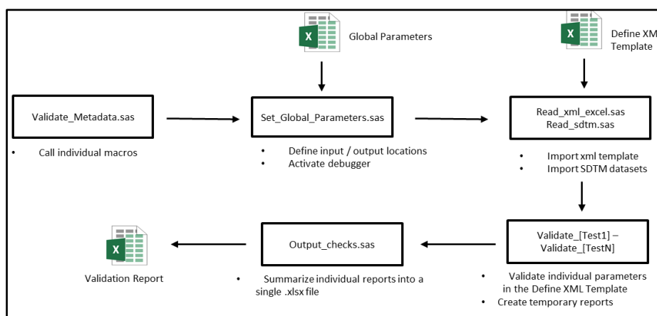
Figure 1: Schematic representation of the workflow used by the validation macro
