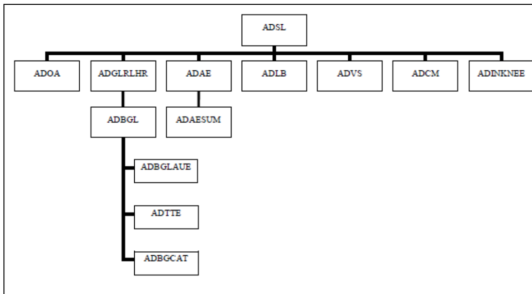
Figure 4: ADaM Data Dependencies
