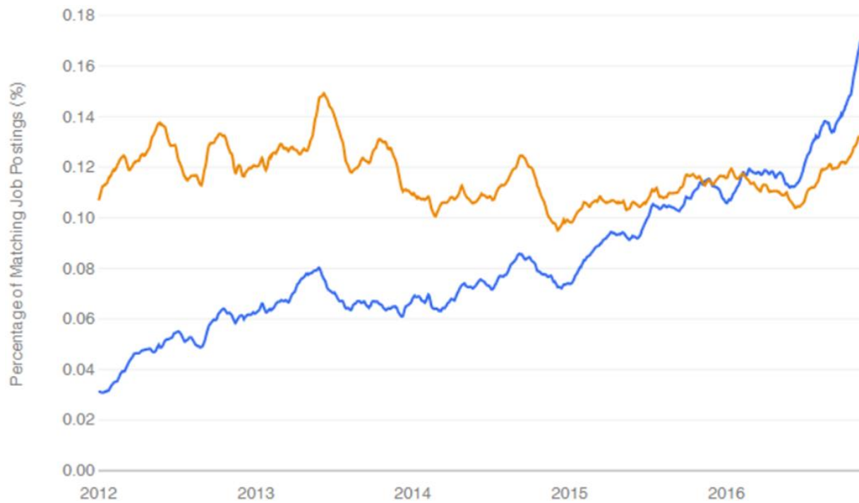
Fig 1. Percentage of Matching job postings (R in Blue, SAS in Orange).
