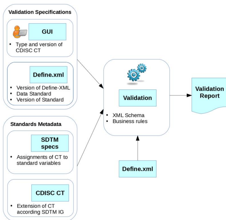
Figure 1. Configurations for define.xml validation
