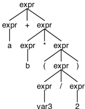
Parse tree
