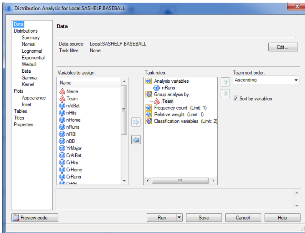
Figure 11. Completed Data for the Distribution Analysis task in Enterprise Guide 7.1.
