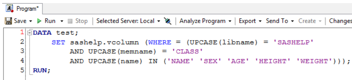
Figure 30. SAS code after formatting by Enterprise Guide 7.1.
