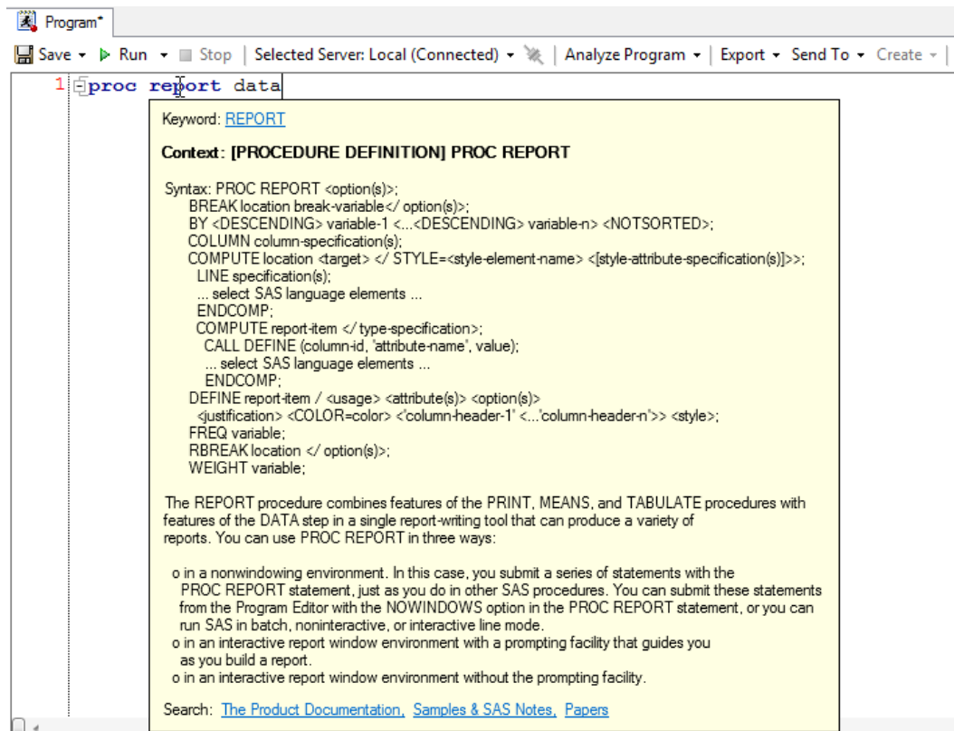
Figure 22. SAS syntax hints and help in Enterprise Guide 7.1.
