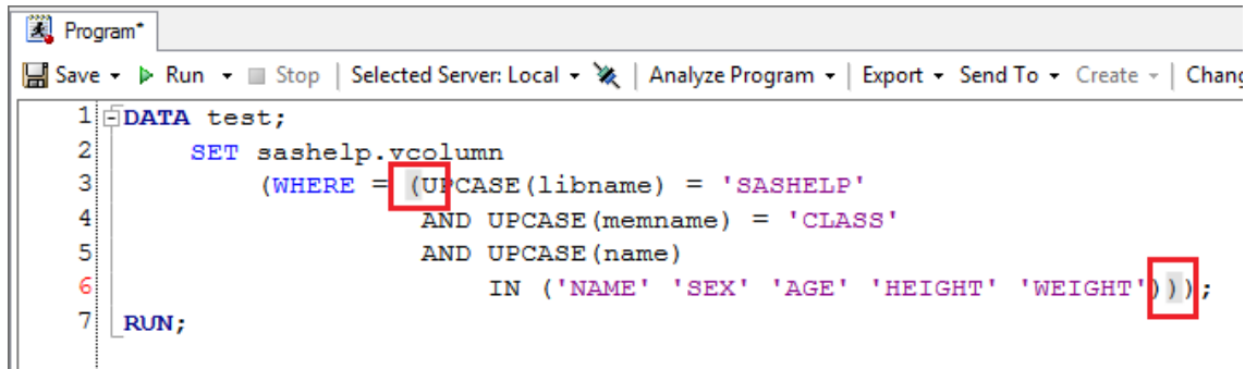
Figure 28. Highlighting matching brackets in Enterprise Guide 7.1.
