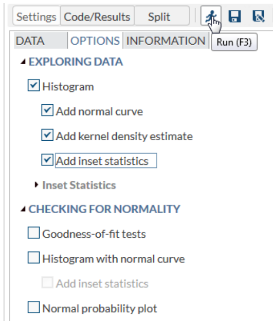
Figure 8. Completed Options for the Distribution Analysis task in SAS Studio.
