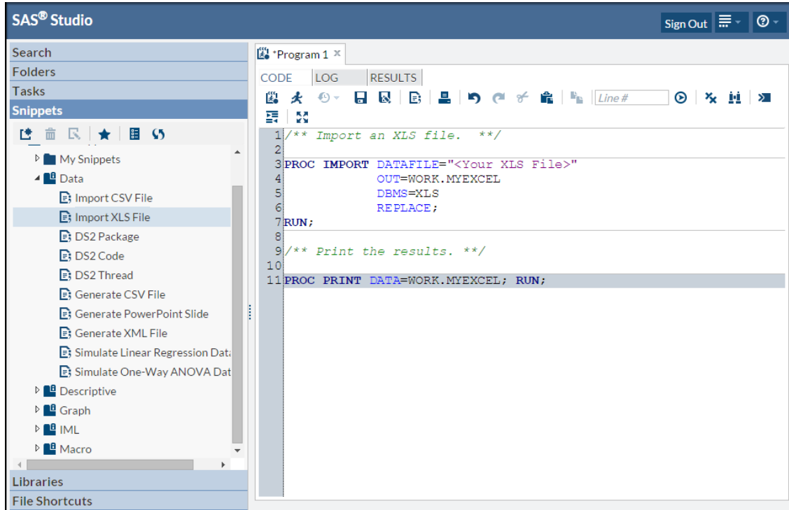
Figure 23. Import XLS File from Data-related Snippets in SAS Studio.
