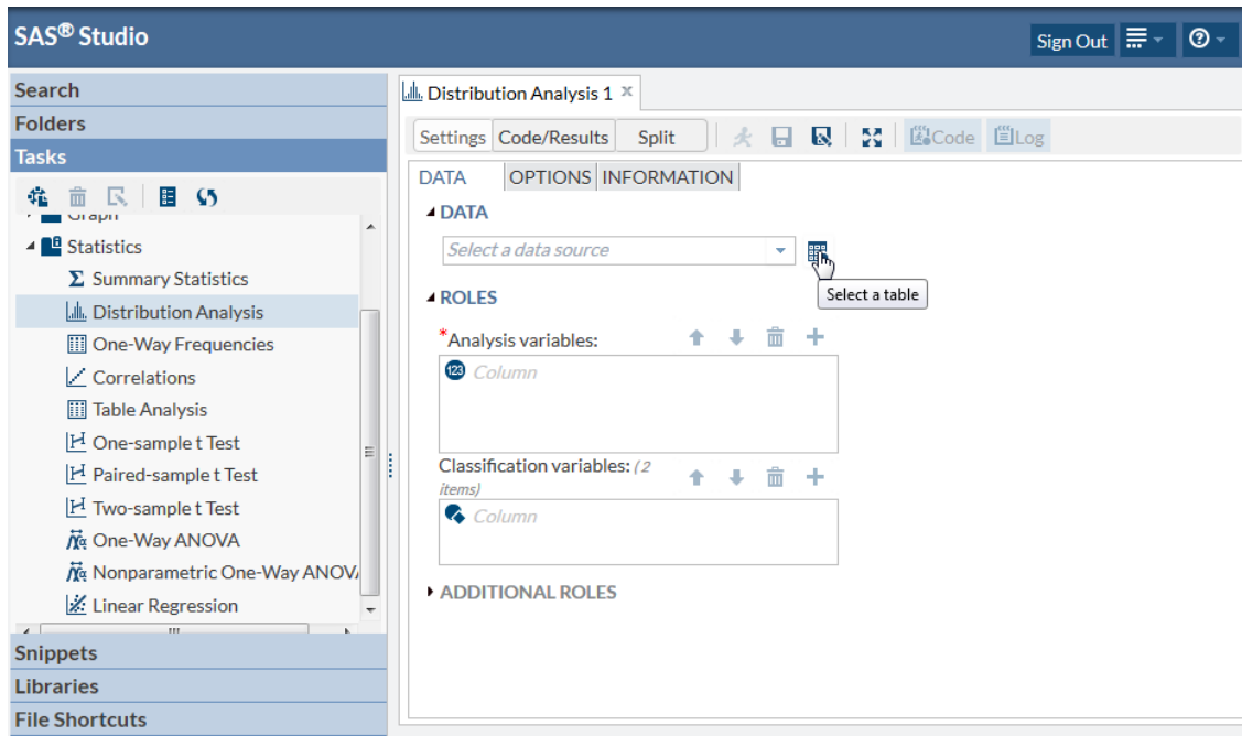
Figure 6. Settings for the Distribution Analysis task in SAS Studio.
