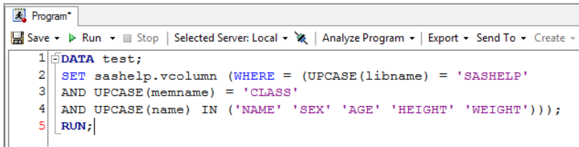
Figure 29. SAS code before formatting by Enterprise Guide 7.1.
