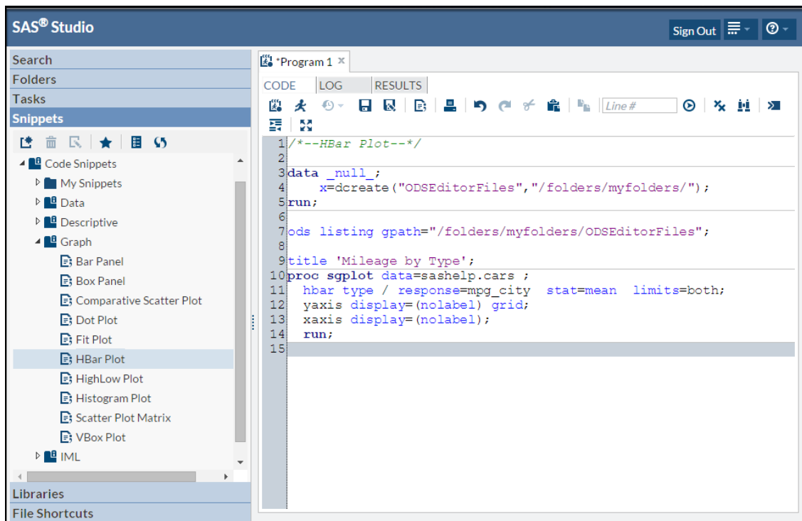
Figure 24. Horizontal Bar chart from Graph-related Snippets in SAS Studio.
