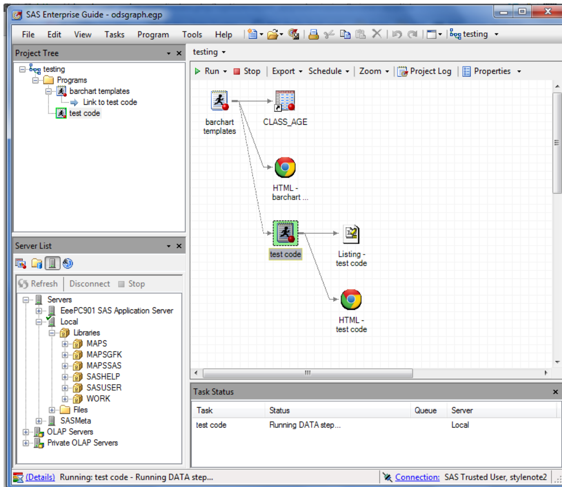
Figure 27. Connected program nodes in Enterprise Guide 7.1.
