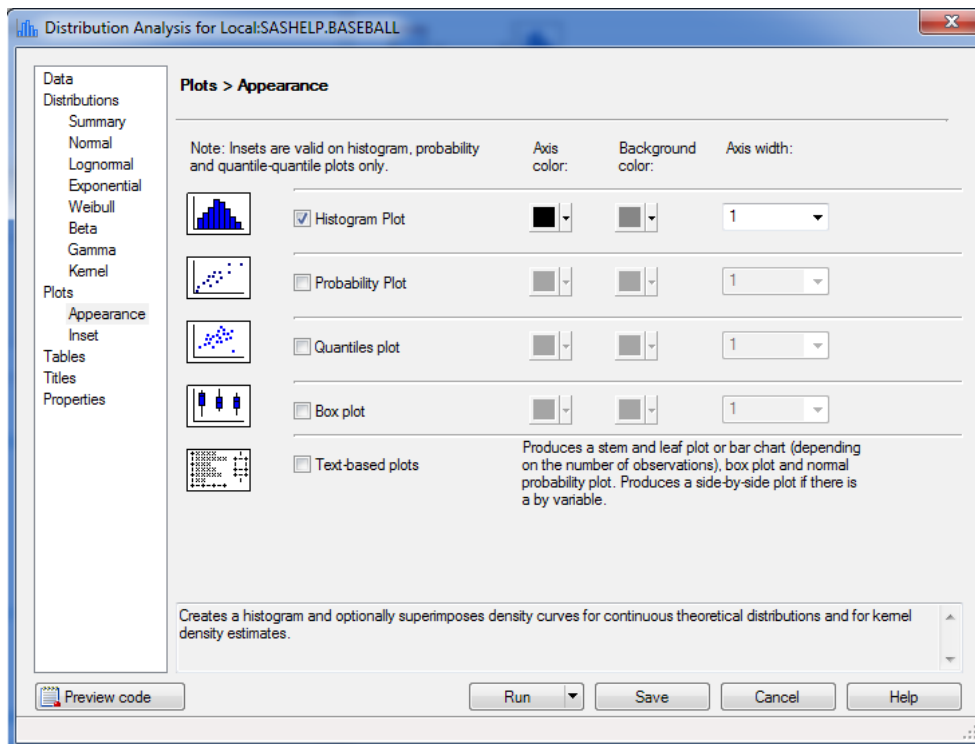
Figure 12. Completed Appearance for the Distribution Analysis task in Enterprise Guide 7.1.
