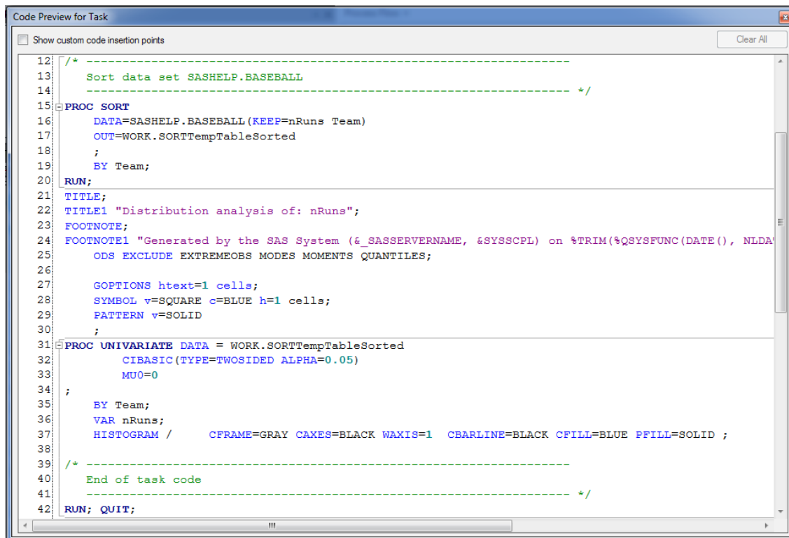
Figure 20. SAS code generated by Distribution Analysis Task in Enterprise Guide 7.1.
