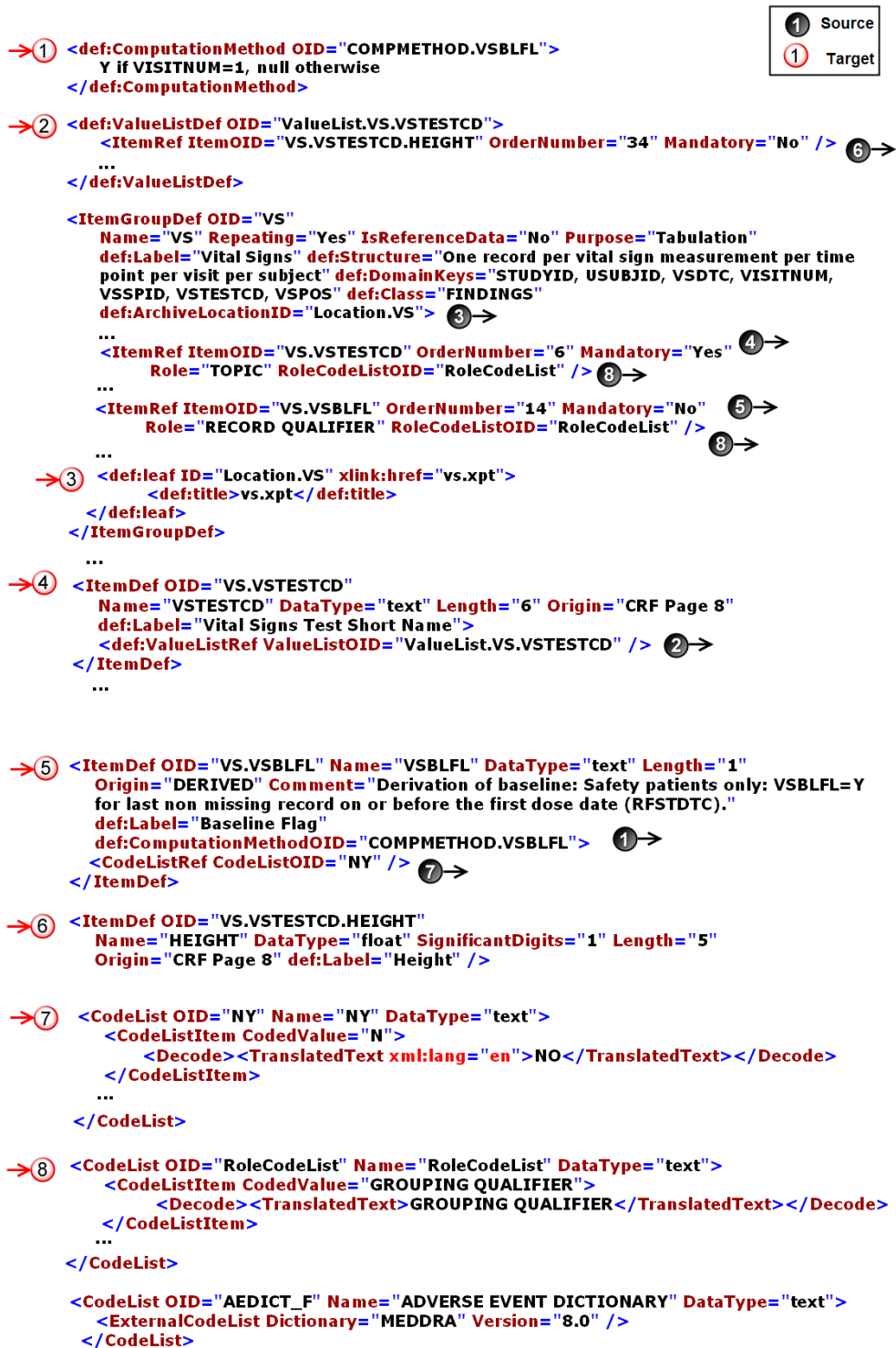
Figure 11: Relations within a define.xml
