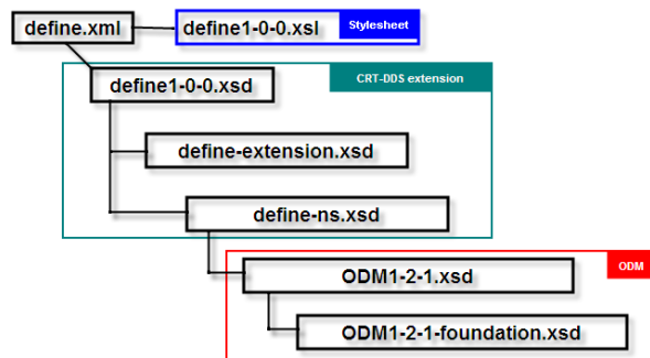
Figure 6: The define.xml (CRT-DDS) and the associated style sheet and schemas
