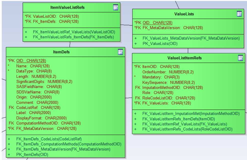
Figure 13: CRT-DDS Datasets related to value level metadata
