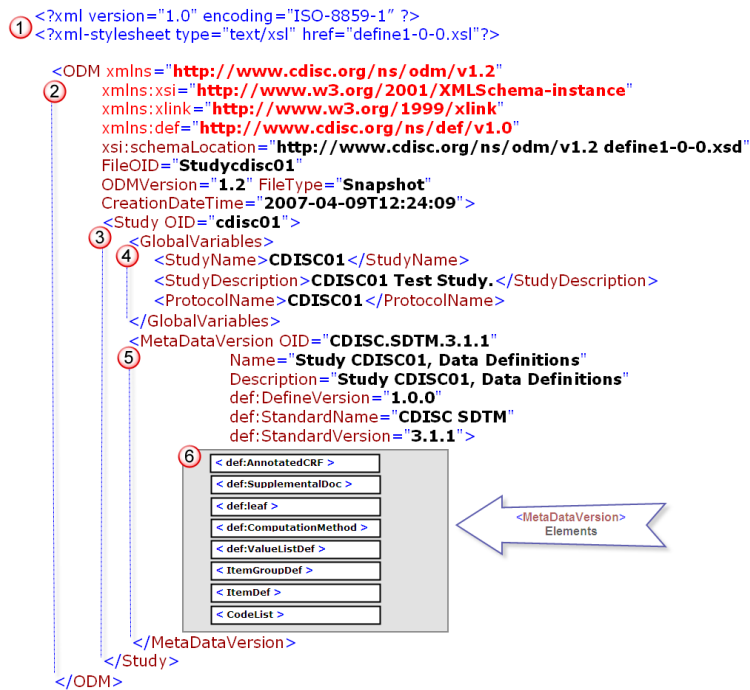
Figure 7: The building blocks of the define.xml (CRT-DDS)
