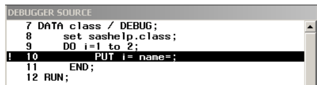
Figure 5 SAS DATA Step Debugger
