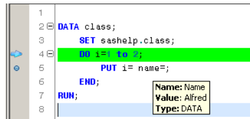
Figure 6 MACUMBA DATA Step Debugger
