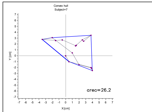
Fig. 3: Convex hull
