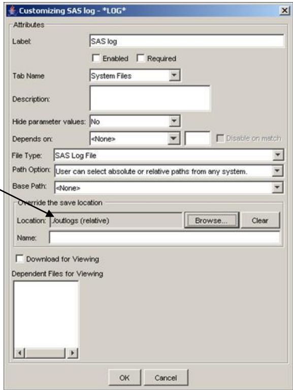
Figure 6: LOG File Written to the './outlogs' Folder
