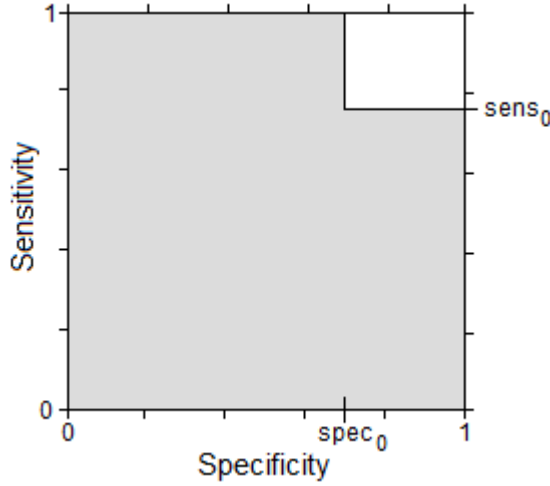
Figure 1. Regions in the (sens, spec) space for a binary test that correspond to unacceptable tests ( H_0 , shaded region) and acceptable tests (unshaded region). (Figure adapted from [3].)
