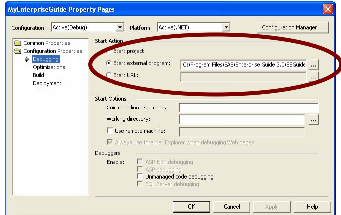
Figure 10: Configuring project properties for debugging
