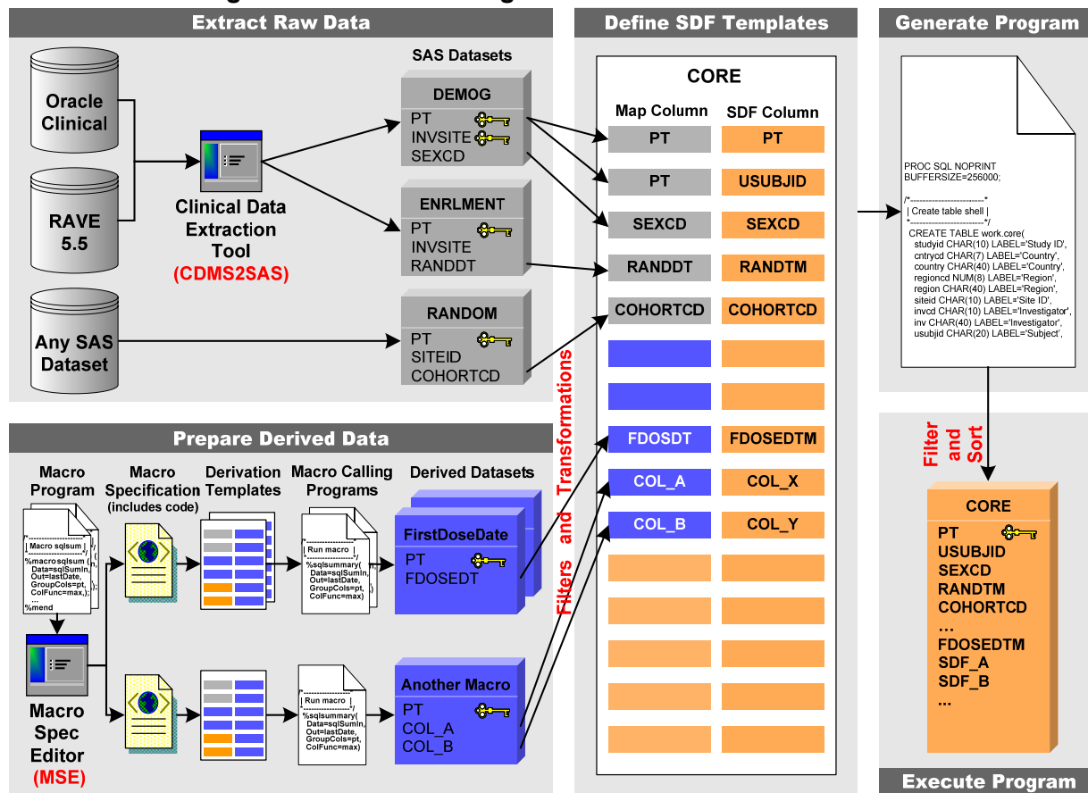
Figure 1: Schematic Diagram of the SDF Creation Process
