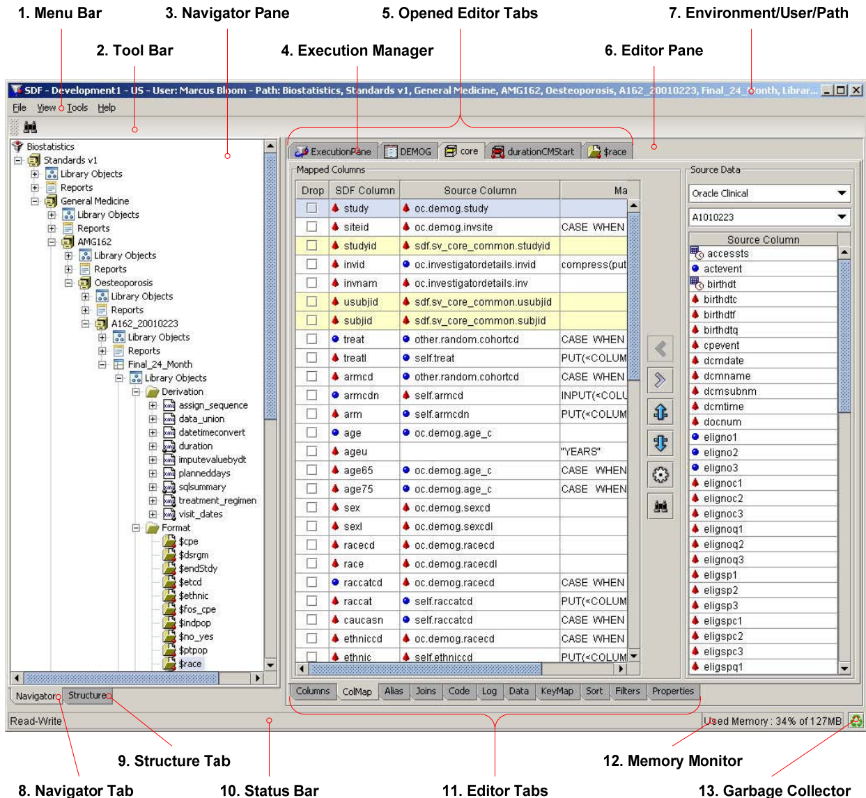
Figure 2: The SDF IDE
