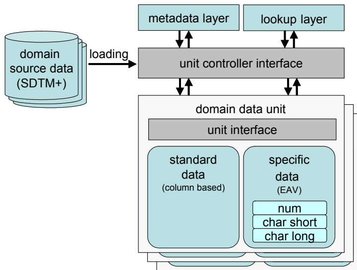
Figure 1. Schematic representation of the proposed D3W data warehouse architecture. The distribution of standard and study-specific data is domain specific. For efficiency reasons, specific data contains separate EAV structures for different data types (num, char short, char long).
