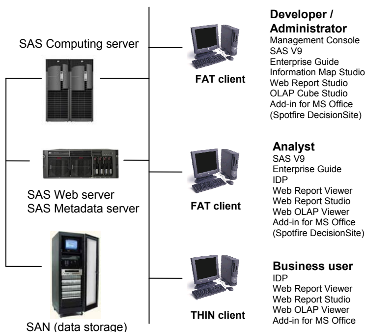
Figure 3. Overview of the proposed hardware and software design of D3W.
