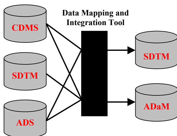
Direct Migration
